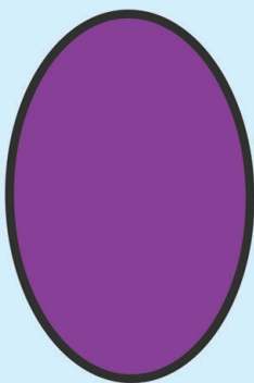
oval
