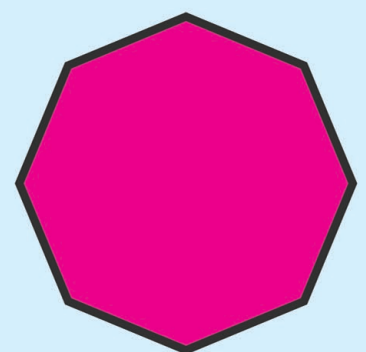
octagon
