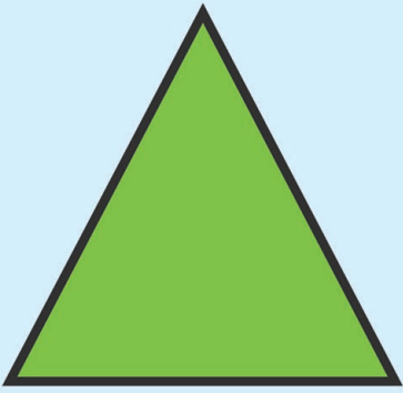
triangle
