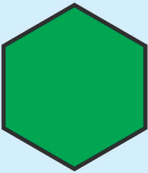
hexagon
