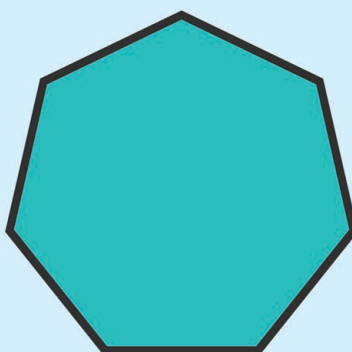
heptagon
